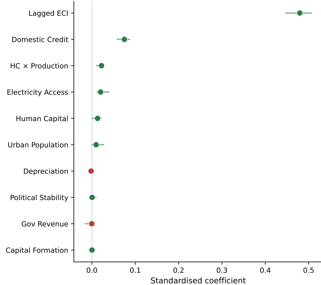
ElasticNet
