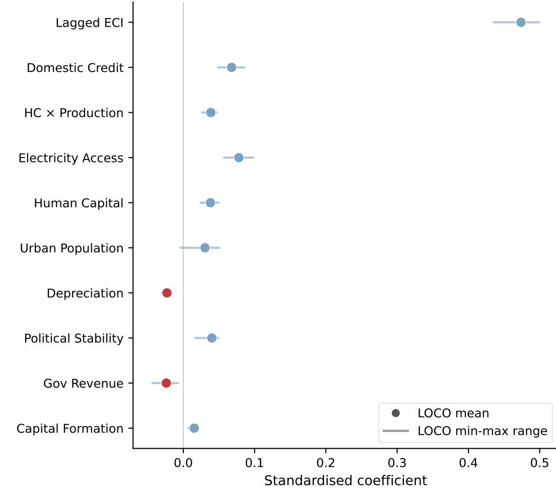
Ridge
